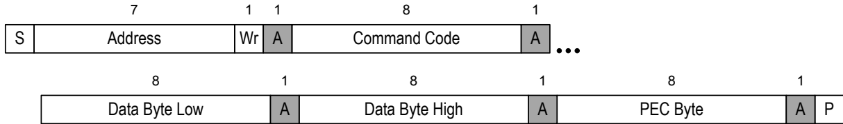
Figure 28: Write Word protocol with PEC
