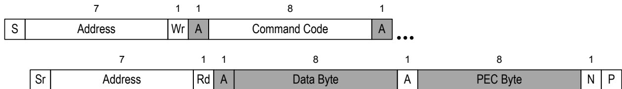
Figure 30: Read Byte protocol with PEC
