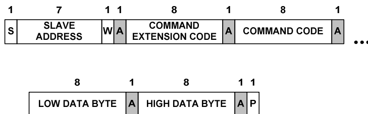
Figure 10. Extended Command Write Word Protocol
