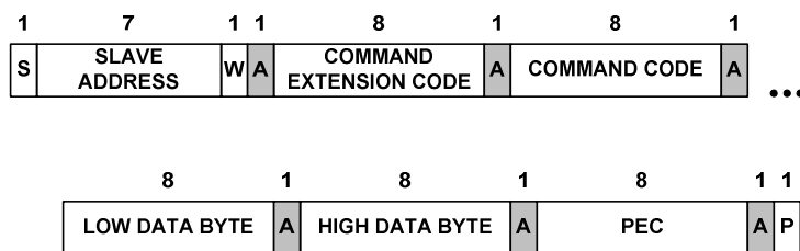
Figure 11. Extended Command Write Word Protocol With PEC
